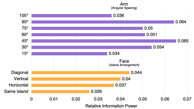
Figure 9. Performance of different transducer pairings.
