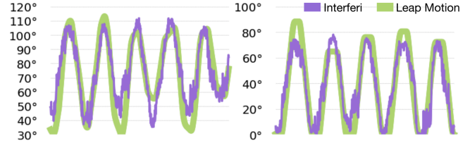
Figure 20. Example thumb (left) and four-finger (right) tracking from one participant, five rounds of data collection. Leap Motion predictions shown in green; Interferi plotted in purple.
